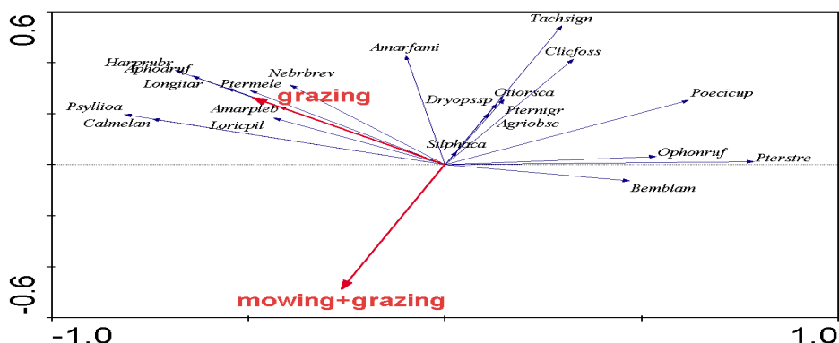
Figure 3 Ordination of beetle species by PCA (activity of species is increasing in the direction of arrow). Amarfami – Amara familiaris , Amarpleb – Amara plebeja , Agriobsc – Agriotes obscurus , Aphodruf – Aphodius rufipes , Bemblam – Bembidion lampros , Calmelan – Calathus melanocephalus , Cliefoss – Clivina fossor , Dryopssp. – Dryops sp., Harprubr – Harpalus rubripes , Longitar – Longitarsus sp., Loricpil – Loricera pilicornis , Nebrbrev – Nebria brevicollis , Otiosca – Otiorhynchus scaber , Poecicup – Poecilus cupreus , Psyllioa – Psylliodes affinis , Ptermele – Pterostichus melanarius , Pternigr – Pterostichus nigrita , Pterstre – Pterostichus strenuus , Silphaca – Silpha carinata , Tachsign – Tachinus signatus .
